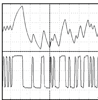
EQUALIZER INPUT AFTER 115ft OF CABLE (TOP) EQUALIZER OUTPUT (BOTTOM)
